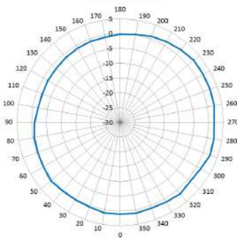
5.0G Horizontal
