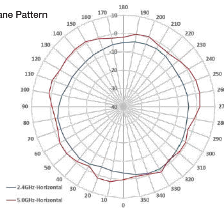
E-Plane Pattern
